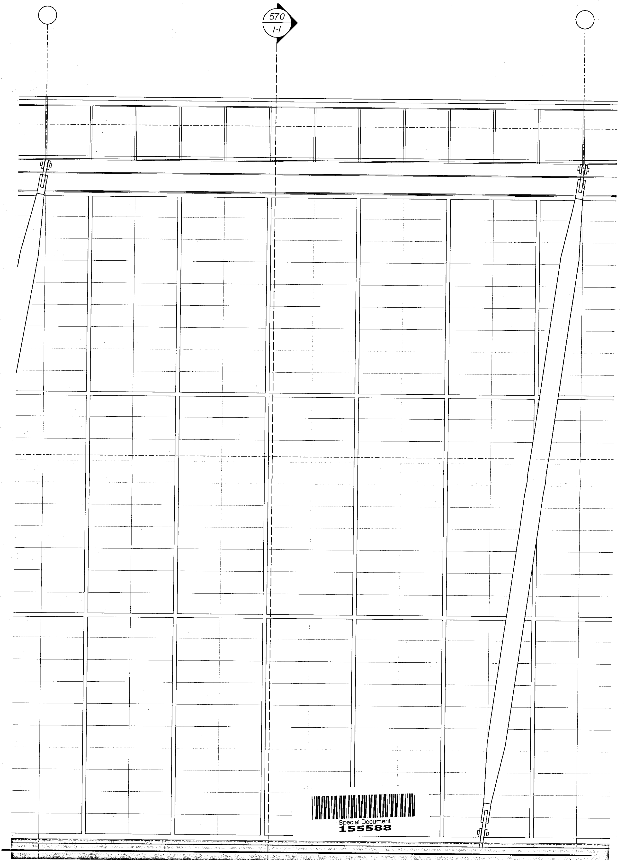
09003-570/02 Multi Purpose Part Elevation Scale: 1:25
